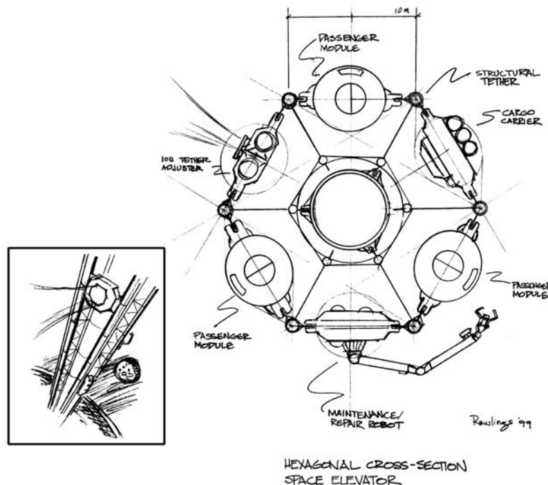
Figure 30. Space elevator cross section. 5 Conceptual cross section of a space elevator showing high-speed passenger modules, cargo carrier, maintenance and repair robot, and a lateral propulsion module for collision avoidance control at any point on the elevator structure. Note also that the cross section of the entire structure is large enough that a direct hit from a large upper stage would not break all of the structural cables. This kind of basic design thinking will need to be put into the space elevator to ensure that catastrophic failure does not occur.
