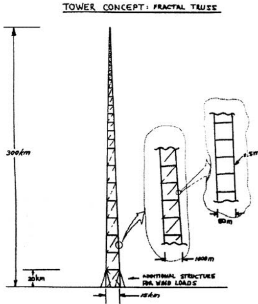
Figure 9. Tall tower concept.
